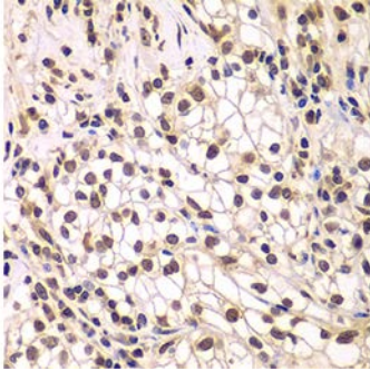
Fig. 3. Immunohistochemistry of paraffin-embedded human kidney cancer using SMARCC1 antibody at dilution of 1:200 (40x lens).
